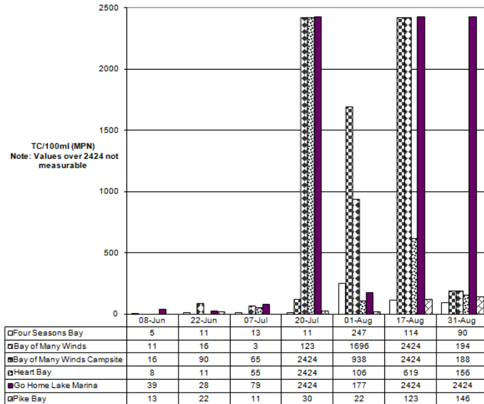
Go Home Lake Total Coliforms 2019
